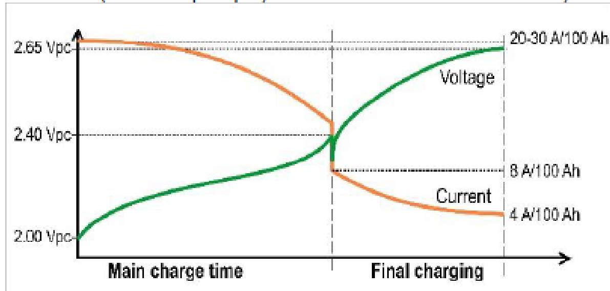
IU1a –characteristics for flooded batteries
