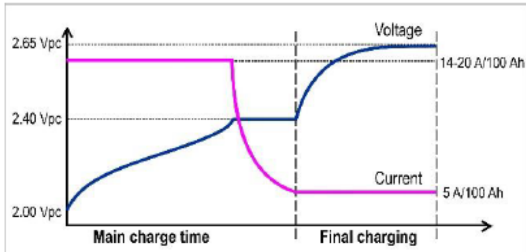
IU1a –characteristics for flooded batteries
